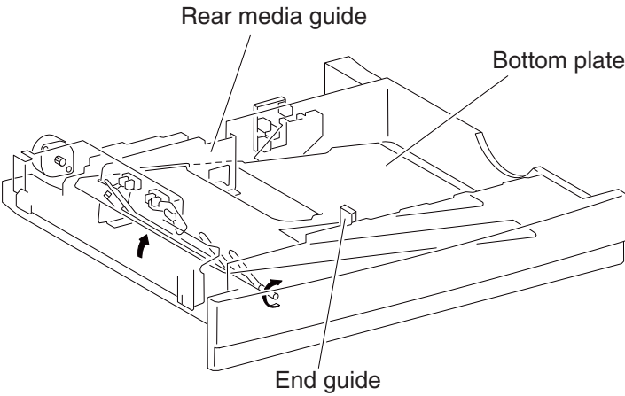
Tray 2 media tray assembly
